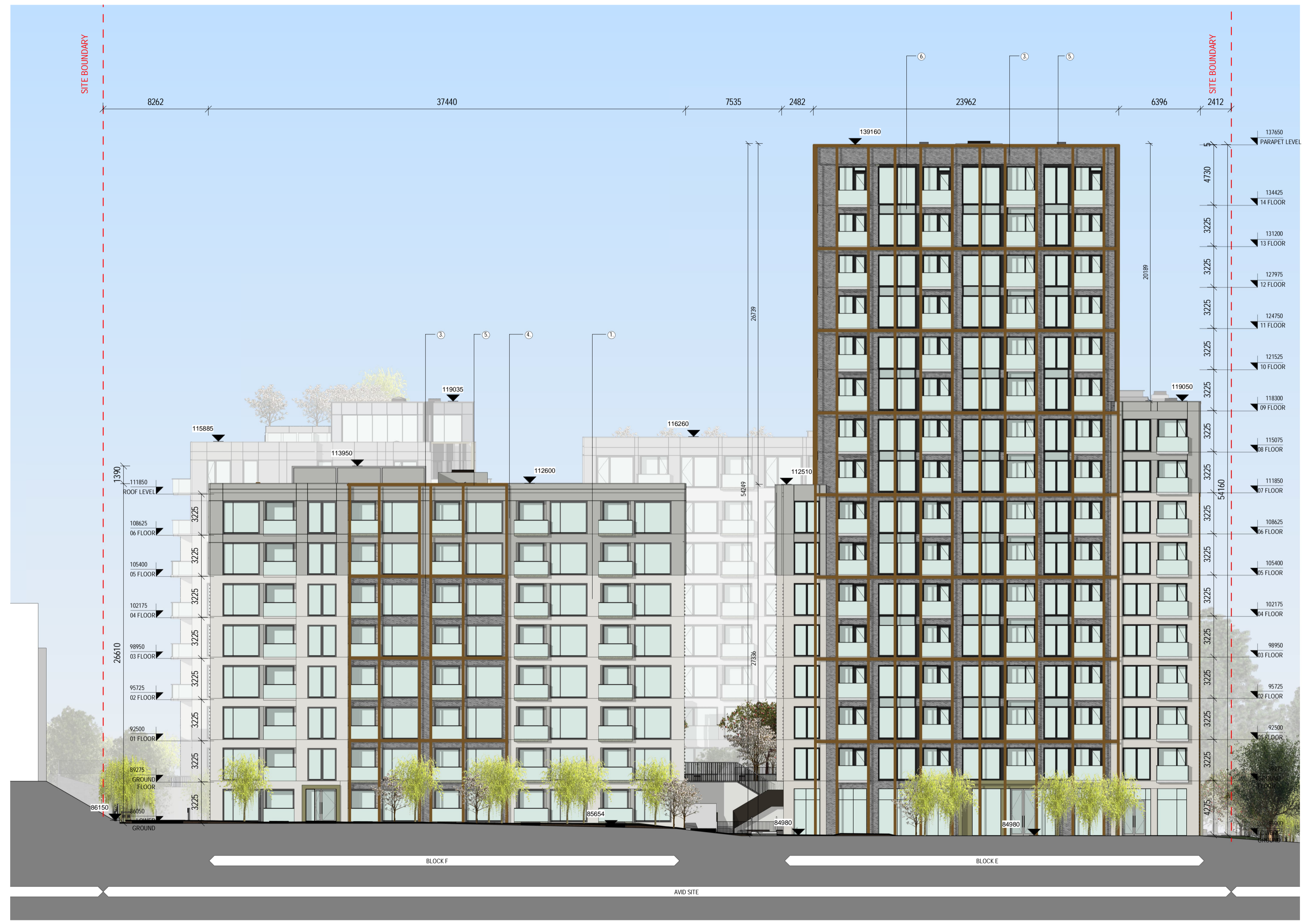
1 PROPOSED SOUTH EAST ELEVATION - AVID SITE 1:200
